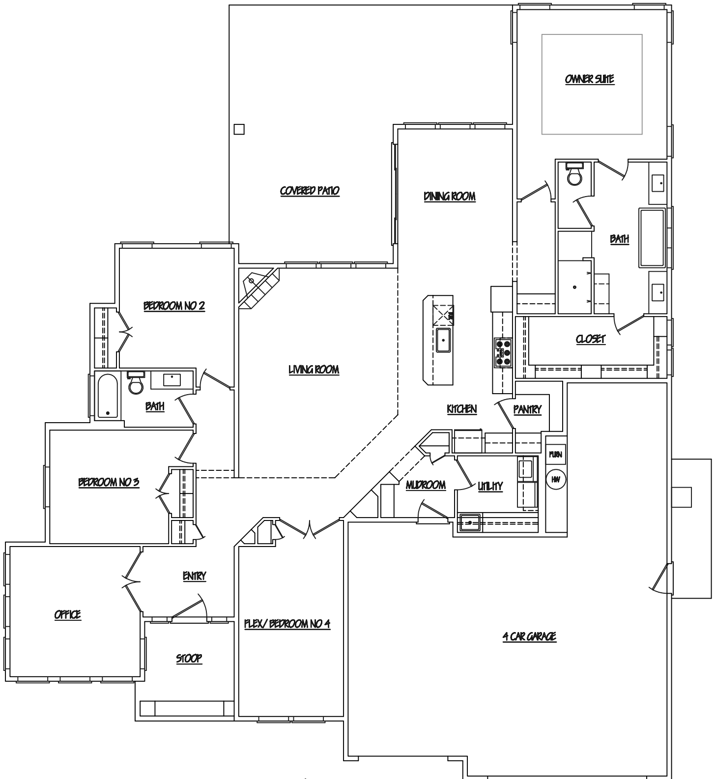
PARKER FLOOR PLAN
